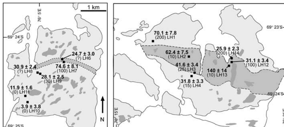
Fig. 5. Cosmogenic nuclide exposure ages \pm 1 \sigma error. The quoted ages are for weathering scenario (1), which assumes that postglacial lowering has no effect on ^{10}\text{Be} concentration. Numbers in brackets refer to the depth of postglacial weathering of the rock surface (in mm).
